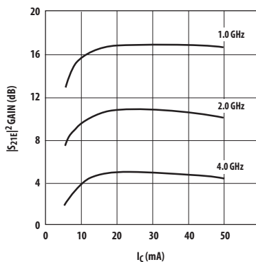
Figure 2. Insertion Power Gain vs. Collector Current and Frequency. V_{CE} = 8\text{ V} .
