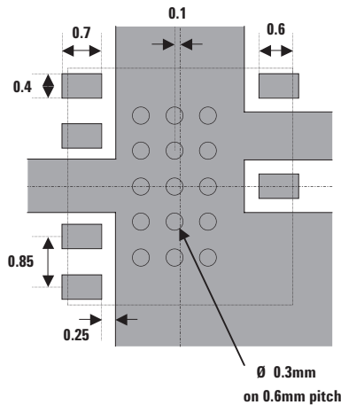
Figure 25. Metallization.
