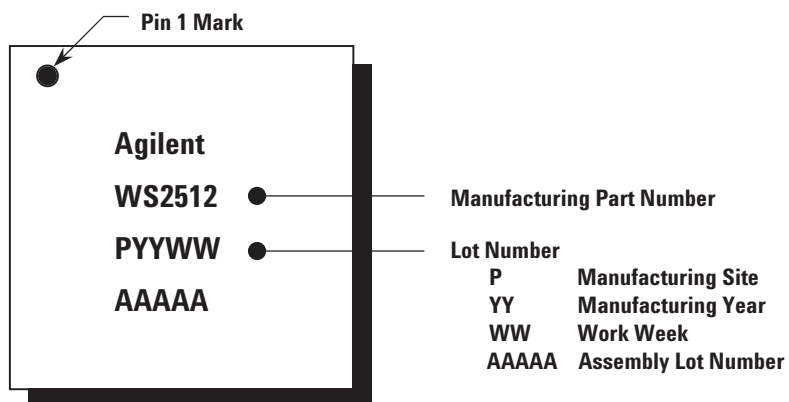
Figure 20. Marking Specification.
