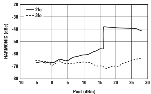
Figure 16. Harmonic Suppression 2 vs. Output Power.
