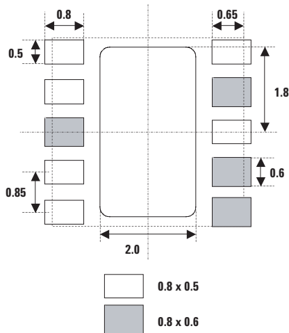
Figure 26. Solder Mask Opening.
