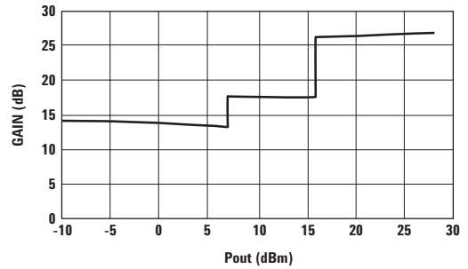
Figure 2. Gain vs. Output Power.
