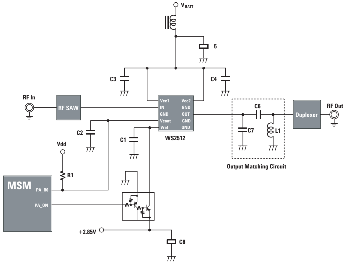
Figure 21. Peripheral Circuit.
