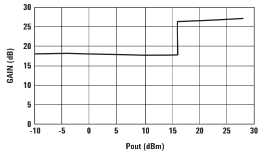
Figure 12. Gain vs. Output Power.
