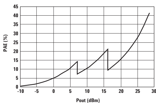
Figure 29. PAE (3-mode control).
