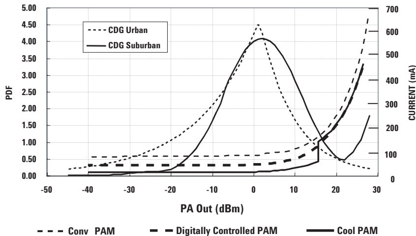
Figure 24. CDMA Power Distribution Function.
