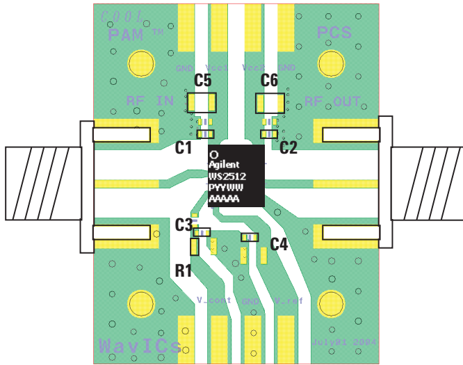
Figure 18. Evaluation Board Assembly Diagram.
