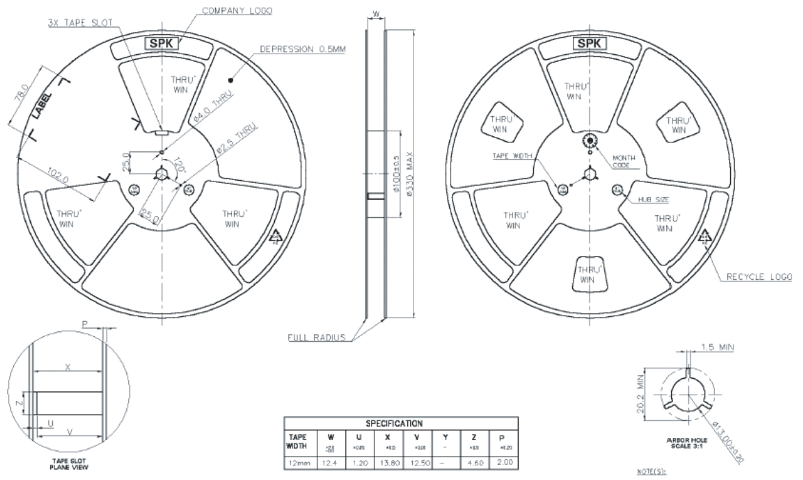
Figure 31. Plastic Reel Format–13"/14".
