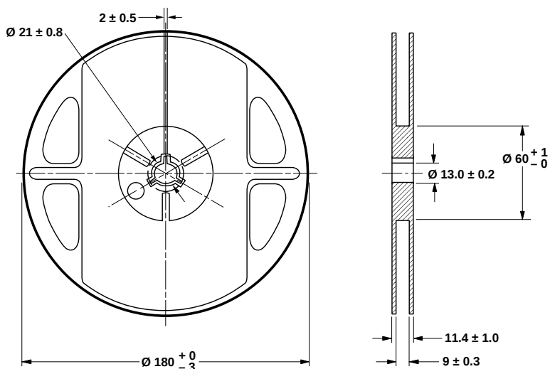
Figure 9. Reel Dimensions.
