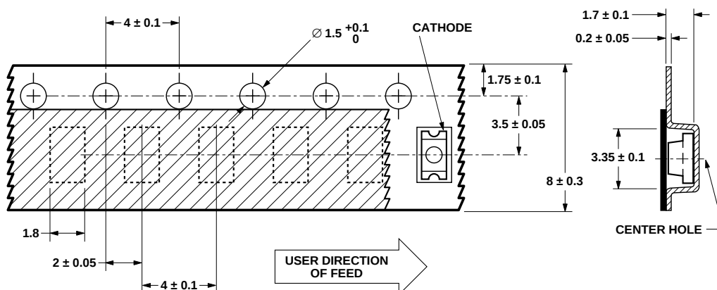
Figure 10. Tape Dimensions.
