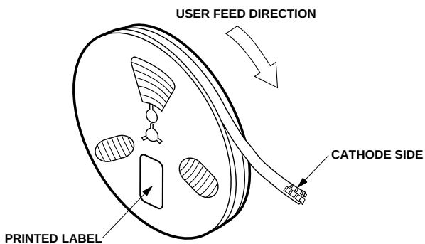
Figure 8. Reeling Orientation.
