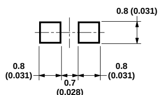
Figure 11. Recommended soldering pattern for HSMx-C192 and HSMx-C196.
