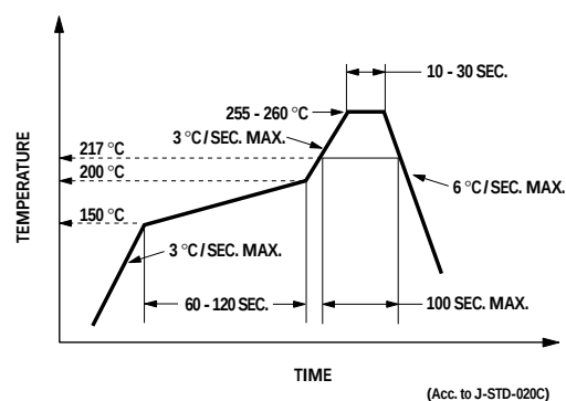
Figure 8. Recommended Pb-free reflow soldering profile.
