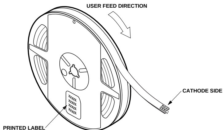
Figure 13. Reeling orientation.
