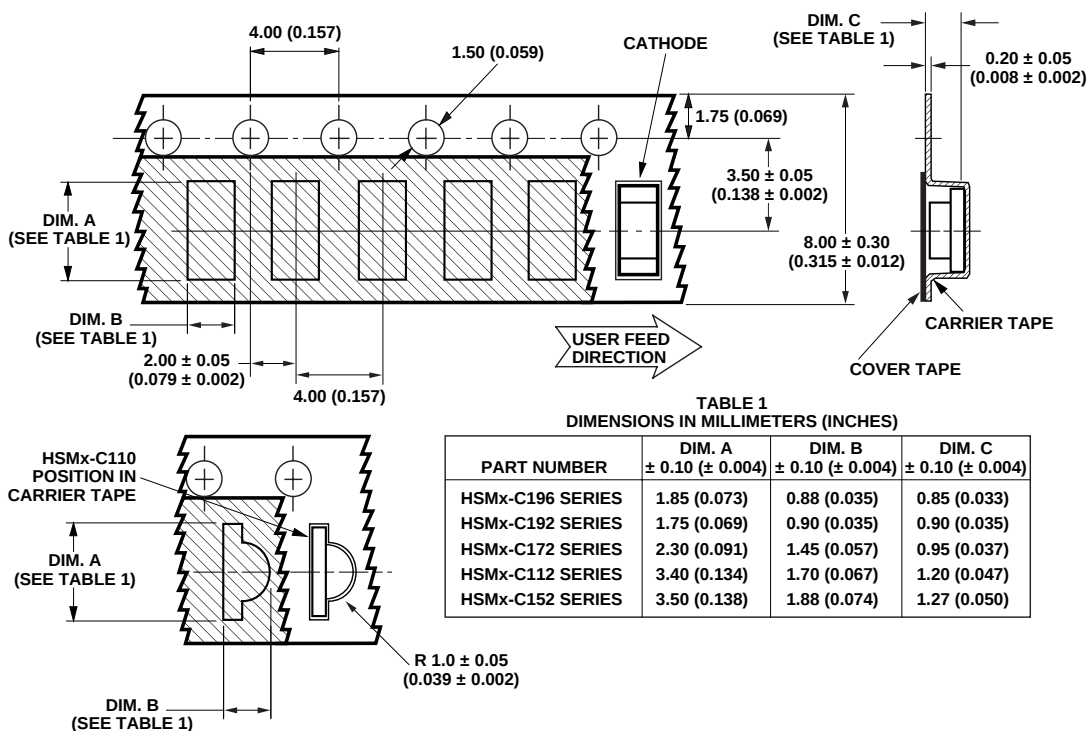
Figure 15. Tape dimensions.
