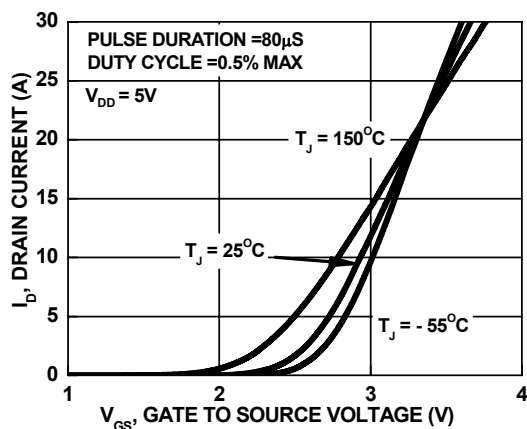
Figure 5. Transfer Characteristics
