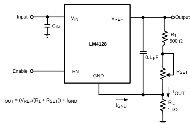
Figure 20. Programmable Current Source
