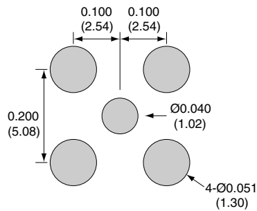
RECOMMENDED FOOTPRINT
