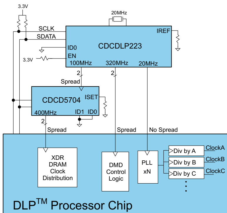
Figure 2. Typical CDCDLP223 Application
