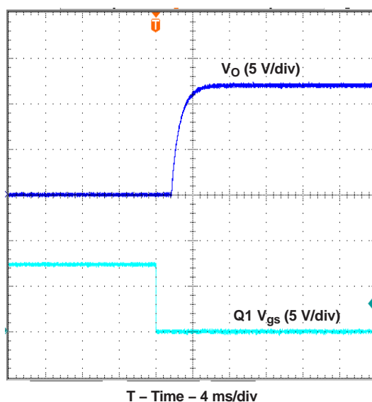
Figure 6. Power Up
