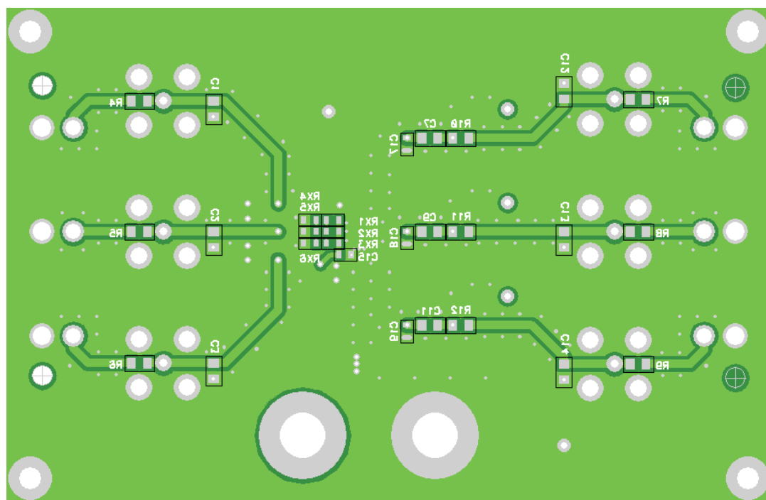
Figure 37. Bottom View
