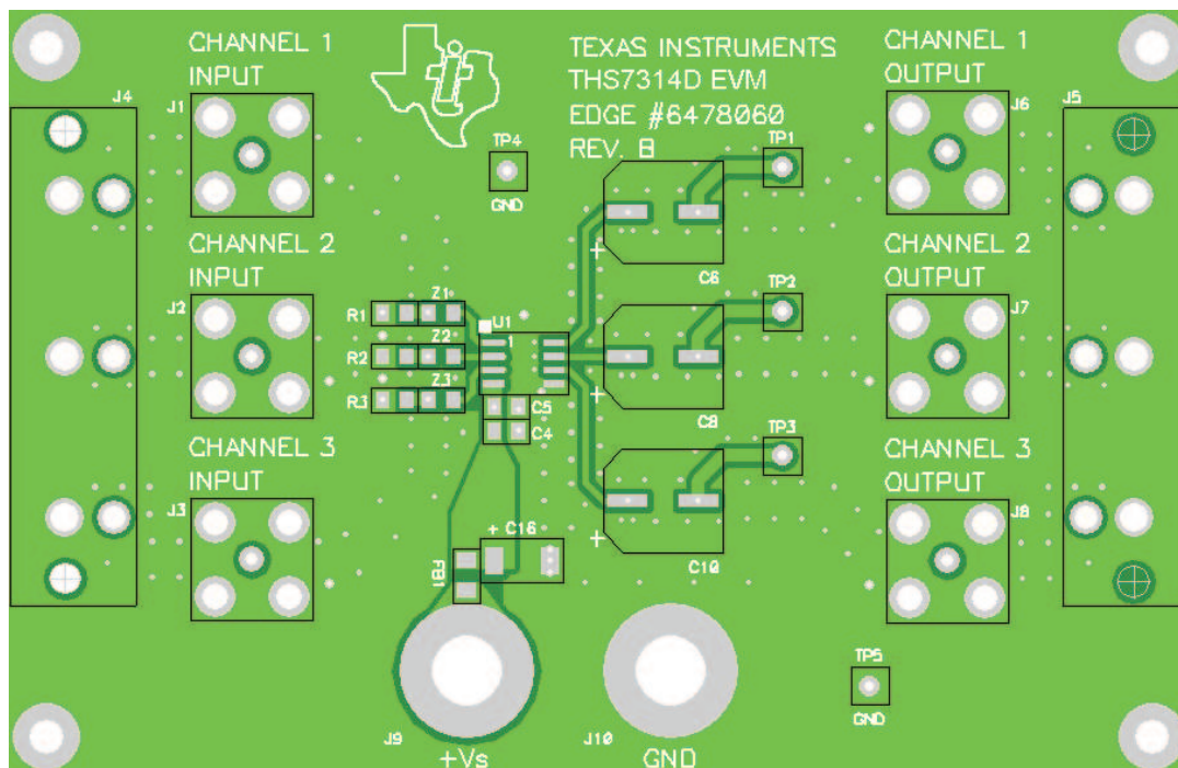
Figure 36. Top View
