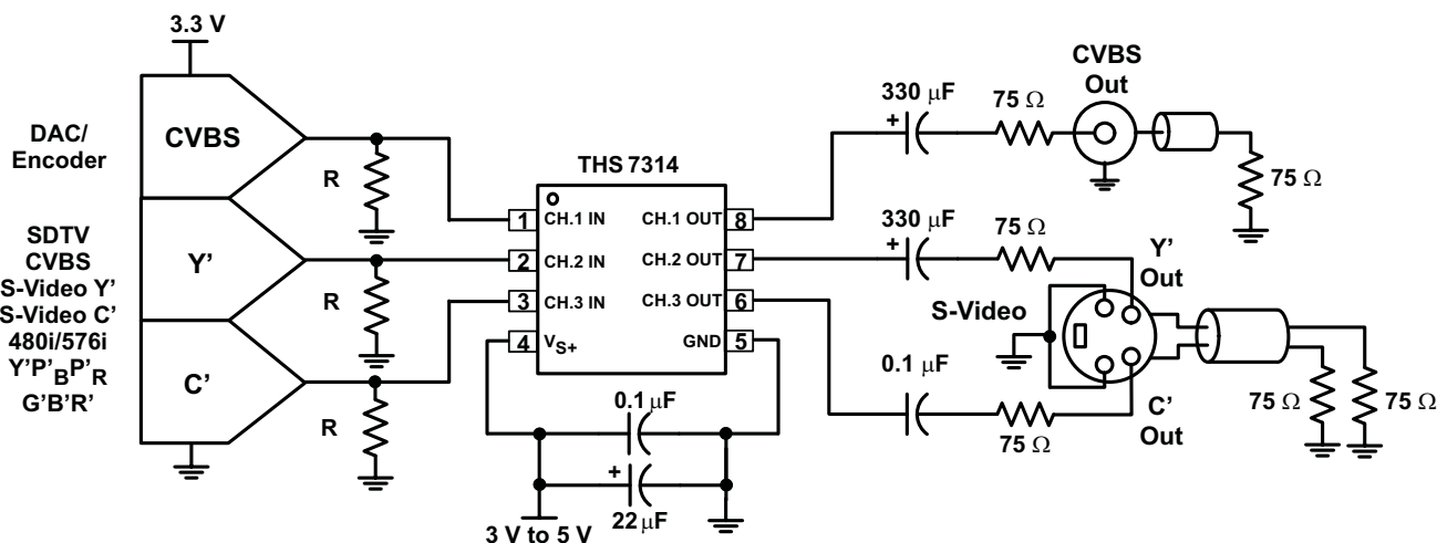
Figure 29. Typical SDTV CVBS/Y'/C' Inputs From DC-Coupled Encoder/DAC With AC-Coupled Line Driving
