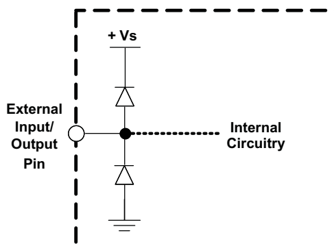
Figure 28. Internal ESD Protection
