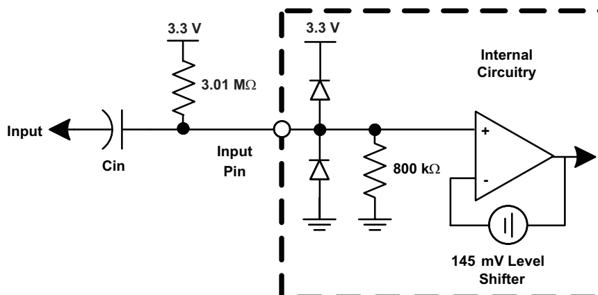
Figure 32. AC-Bias Input Mode Circuit Configuration
