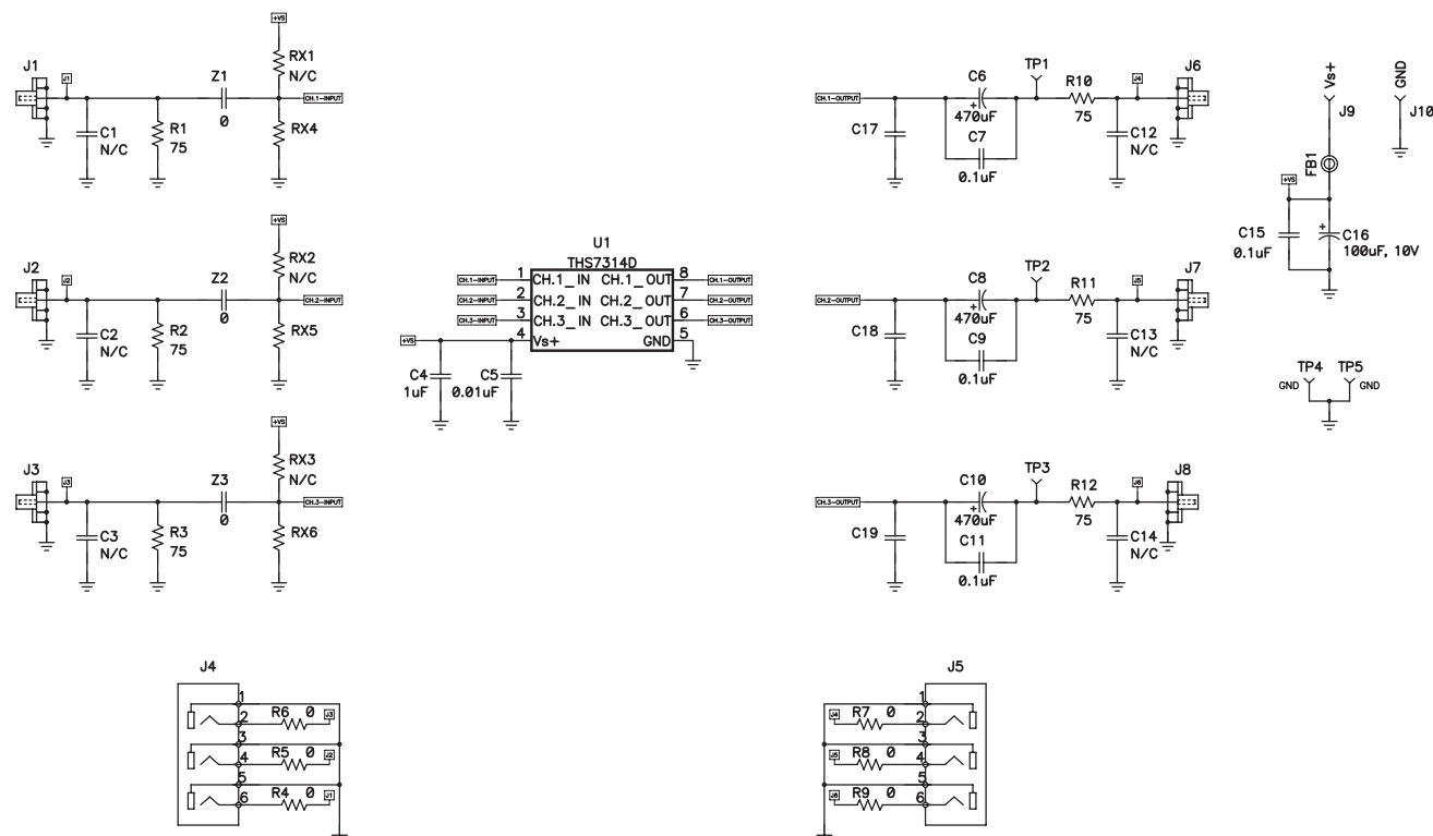
Figure 35. THS7314 Schematic
