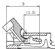
SECT. X-X
