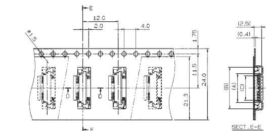
SECT. E-E
