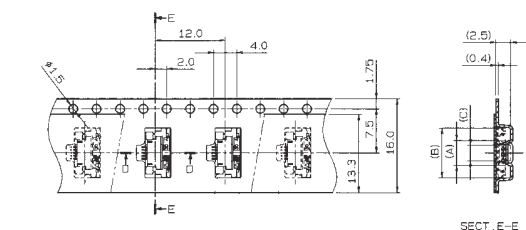
SECT. E-E
