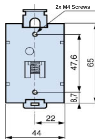
Bracket (DR4 & DR7 Assemblies) (millimeters)
