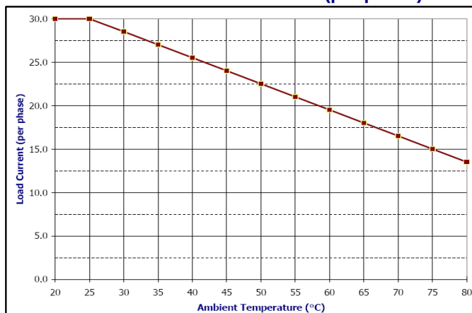
DR34xxx & DR37xxx Series (per phase)
