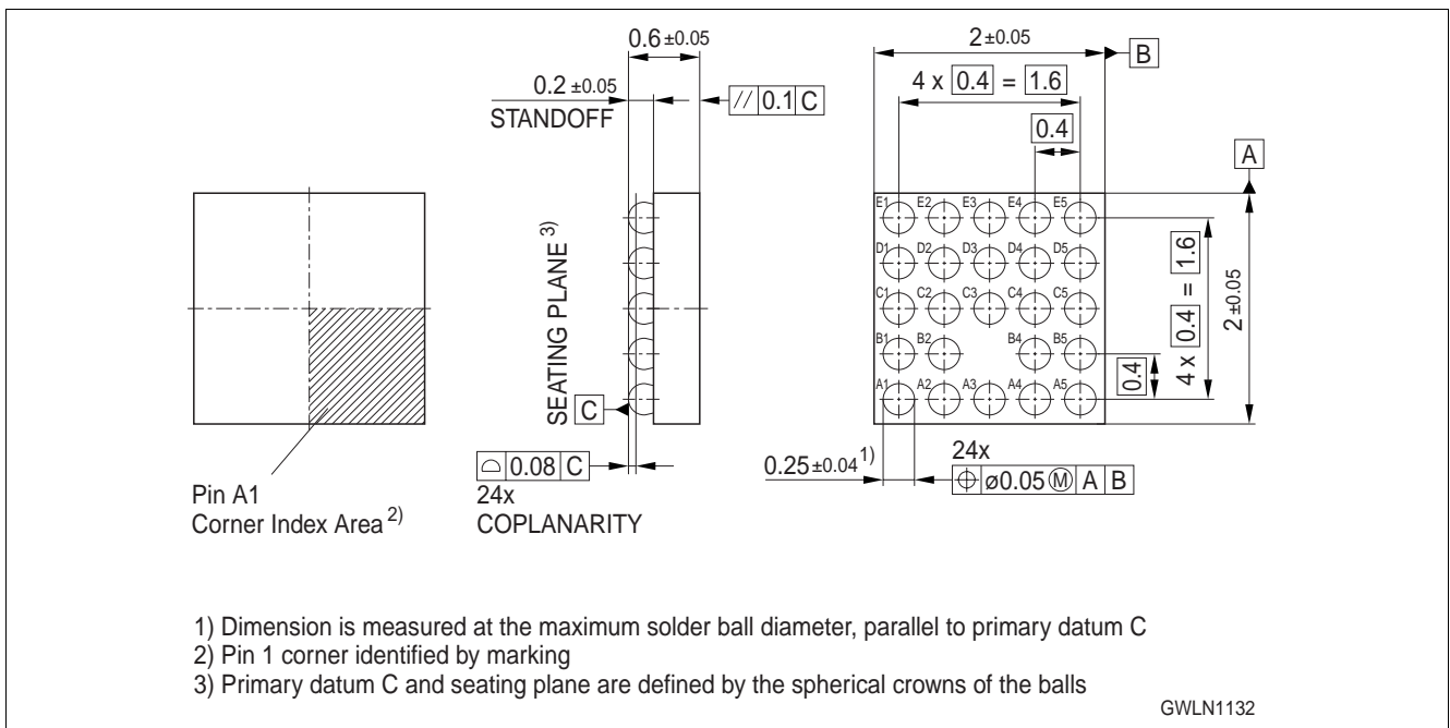
Figure 5 Package WLP-24-2
