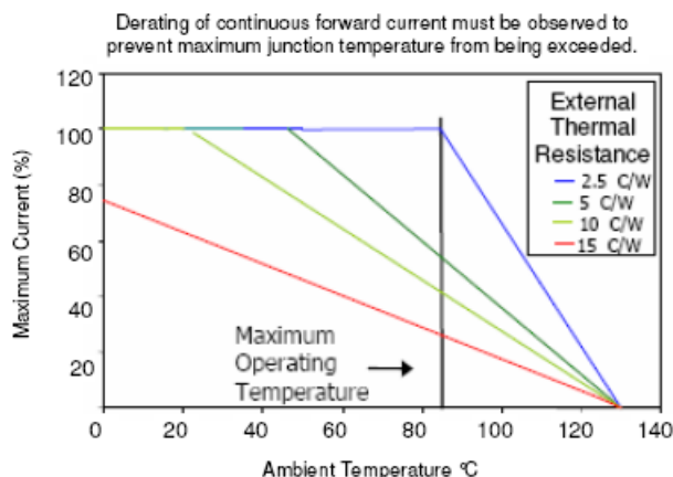
Derating Curves - Blue, Green and White LEDs
