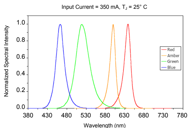
Wavelength Characteristics
