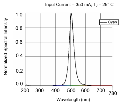
Wavelength Characteristics
