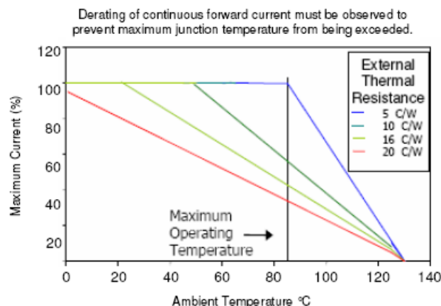
Derating Curves - Amber and Red LEDs
