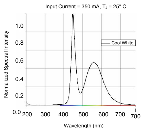
Wavelength Characteristics
