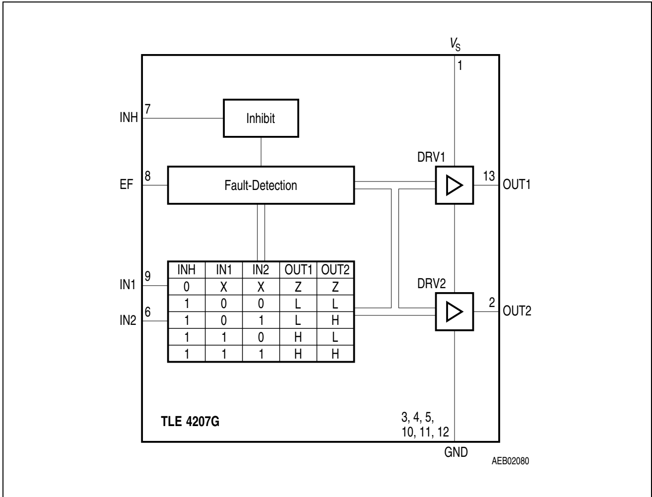
Figure 2 Block Diagram
