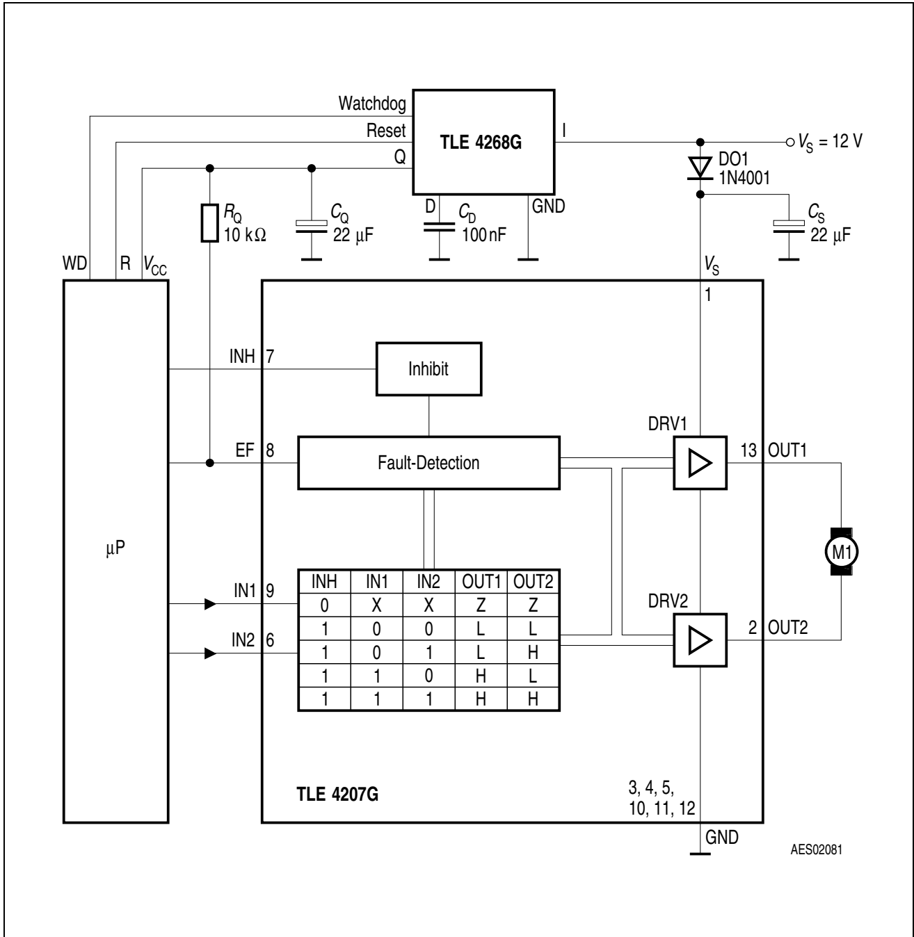
Figure 3 Application Circuit
