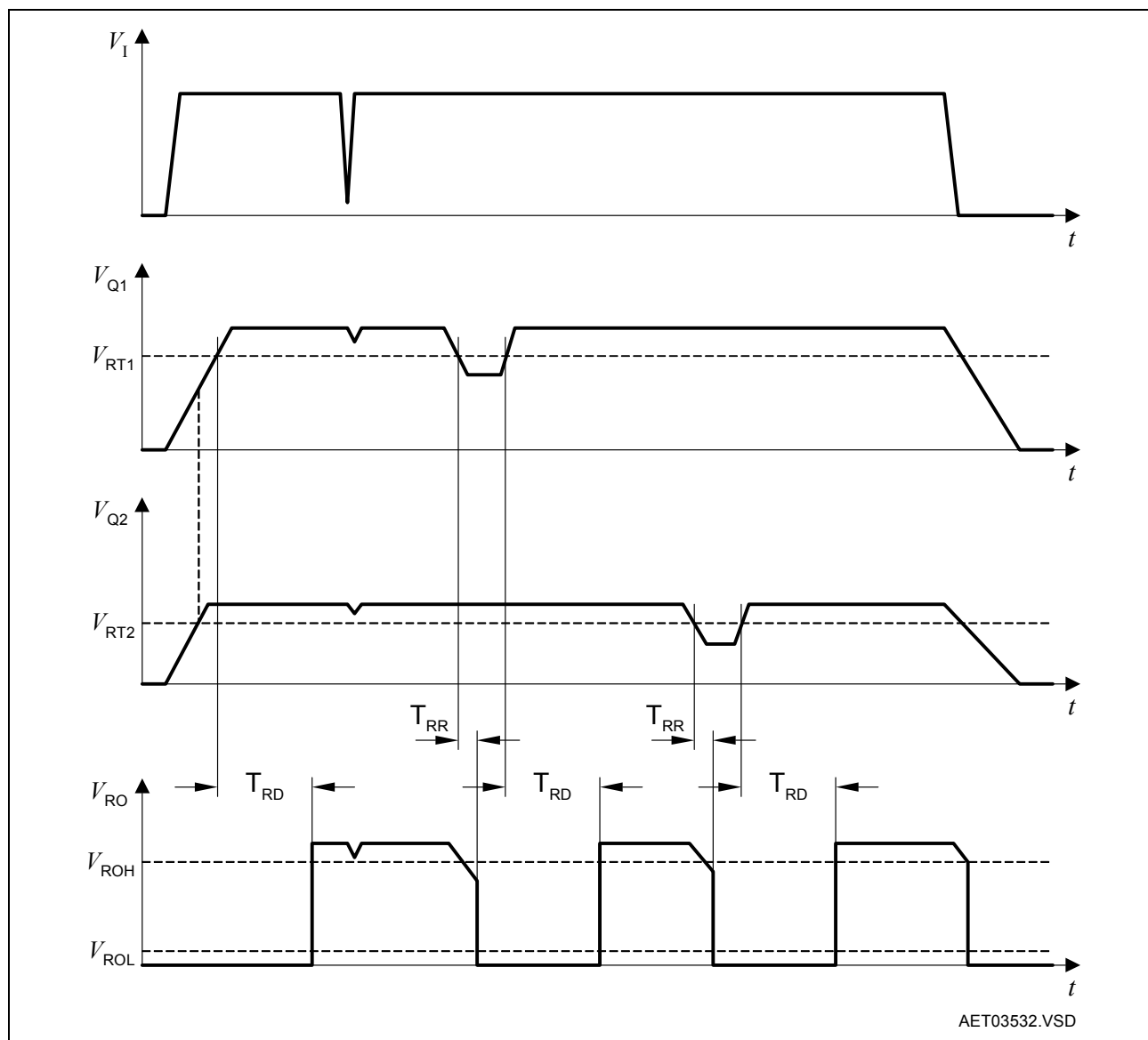
Figure 5 Reset Function and Timing Diagram
