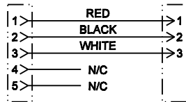
S5F3M WIRING DIAGRAM
