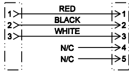
S3F5M WIRING DIAGRAM
