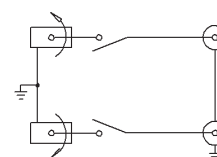
NON-NORMALLED NON-TERMINATED
