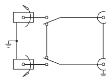
NORMALLED NON-TERMINATED
