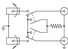
NORMALLED TERMINATED
