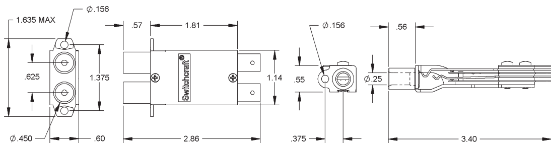
VIDEO JACK
