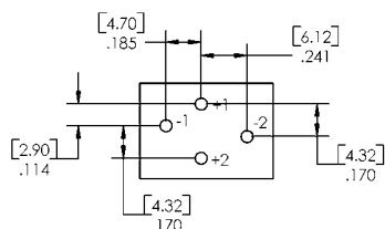
[PC] TERMINALS
