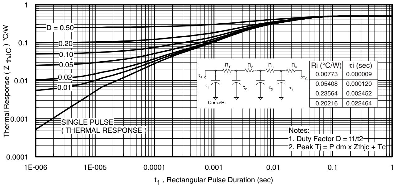
Fig 15. Maximum Effective Transient Thermal Impedance, Junction-to-Case
