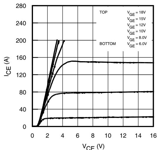
Fig 2. Typical Output Characteristics @ 75°C
