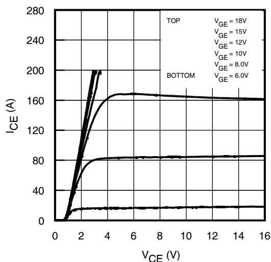
Fig 1. Typical Output Characteristics @ 25°C
