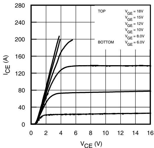
Fig 3. Typical Output Characteristics @ 125°C
