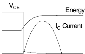
Fig 21b. t_{st} Test Waveforms
