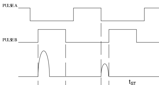
Fig 21c. E_{PULSE} Test Waveforms
