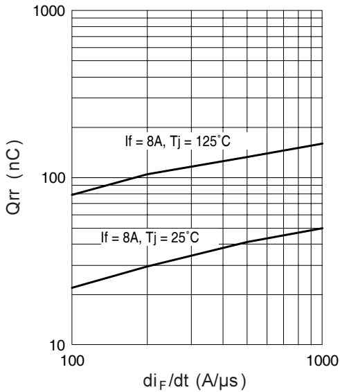
Fig. 19 - Typical Stored Charge vs. di_F/dt
