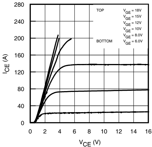
Fig 3. Typical Output Characteristics @ 125^\circ\text{C}
