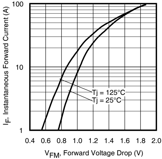
Fig. 17 - Typical Forward Voltage Drop Characteristics
