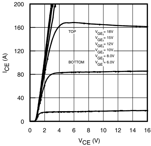
Fig 1. Typical Output Characteristics @ 25^\circ\text{C}
