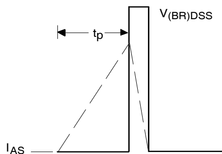
Fig 19b. Unclamped Inductive Waveforms
