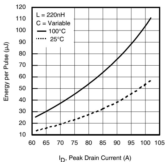
Fig 6. Typical E_{PULSE} vs. Drain Current
