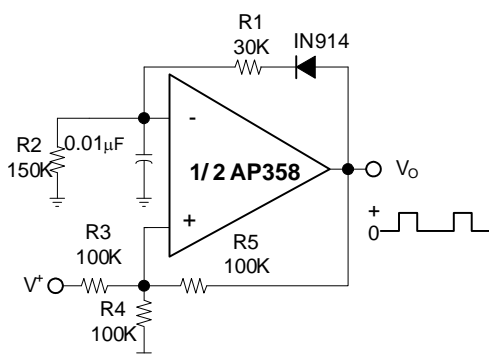
Pulse Generator
