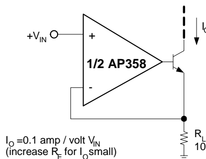
High Compliance Current Sink
