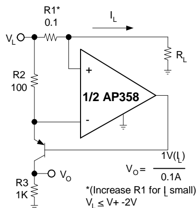
Current Monitor
