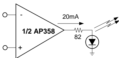
LED Driver
