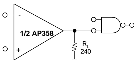
Driving TTL
