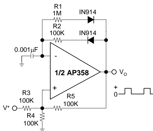
Pulse Generator
