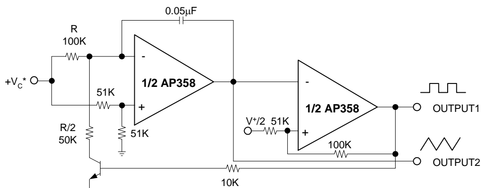
Voltage Controlled Oscillator (VCO)
