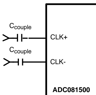
Figure 37. Differential (LVDS) Input Clock Connection
