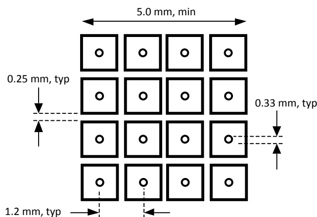
Figure 39. Recommended Package Land Pattern
