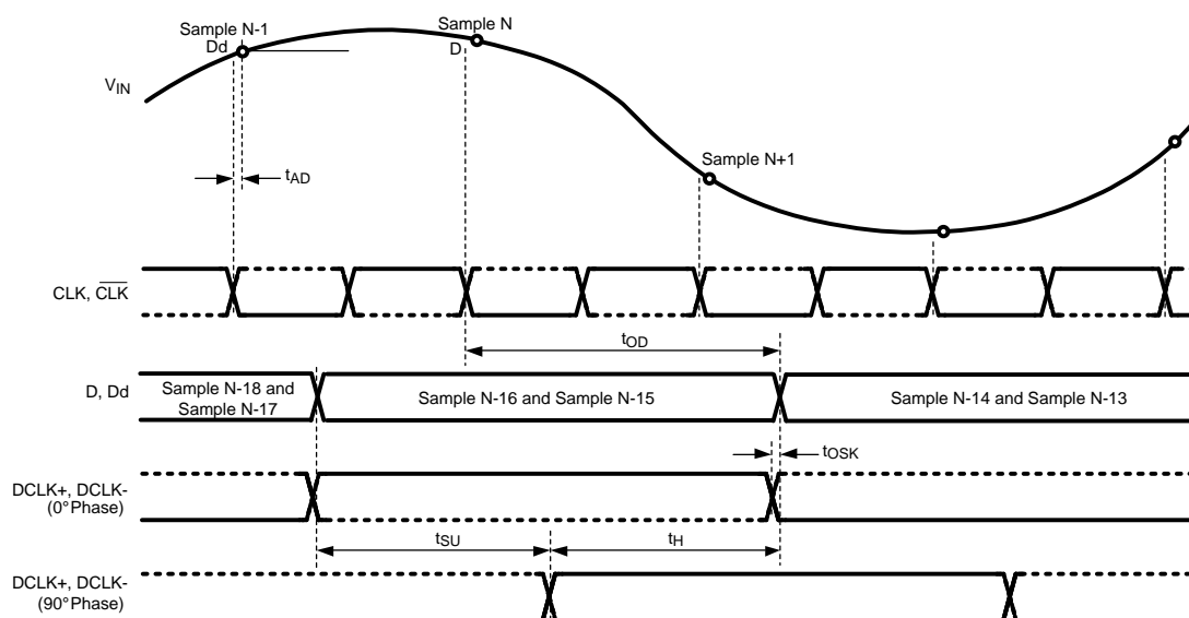
Figure 3. ADC081500 Timing — DDR Clcking
