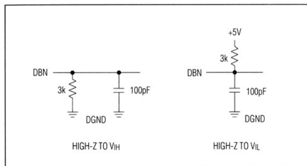
Figure 3. Load Circuits for Access Time Test ( t_{11} )
