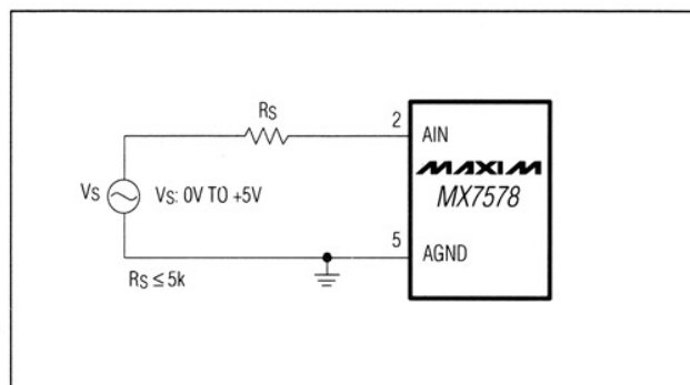
Figure 11. Unipolar 0V to +5V Operation
