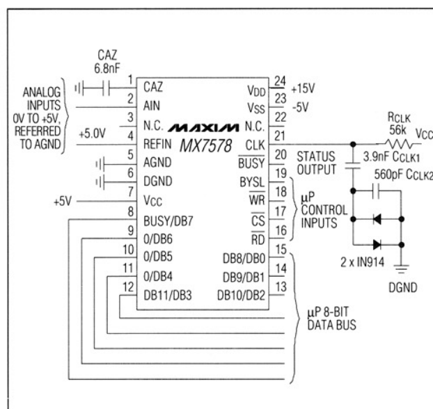
Figure 5. MX7578 Operational Diagram
