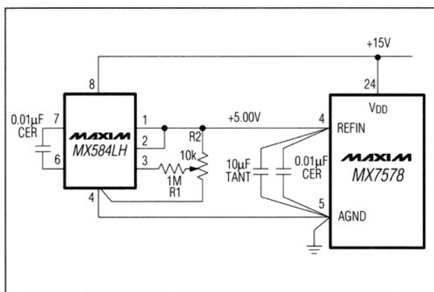
Figure 16. MX584LH as Reference Generator
