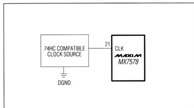
Figure 8. External Clock Operation
