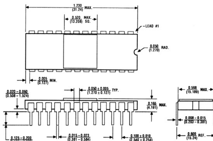
24 Lead Ceramic Sidebraz (DG)
