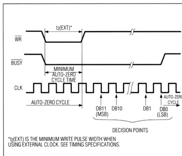
Figure 9. Operating Waveform – External Clock
