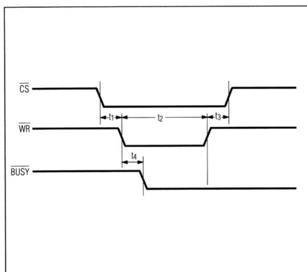
Figure 1. Start Cycle Timing
