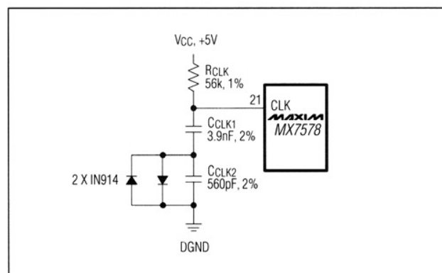
Figure 6. Circuitry Required for Internal Clock Operation
