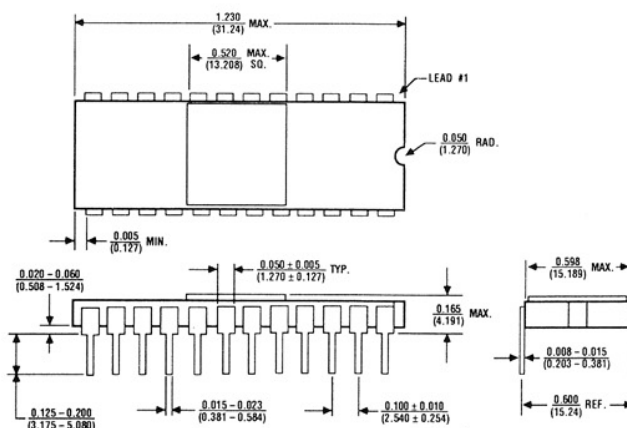
24 Lead Ceramic Sidebraze (DG)
