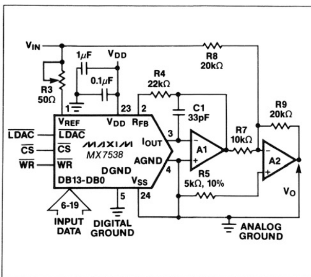
Figure 5. Bipolar Operation
