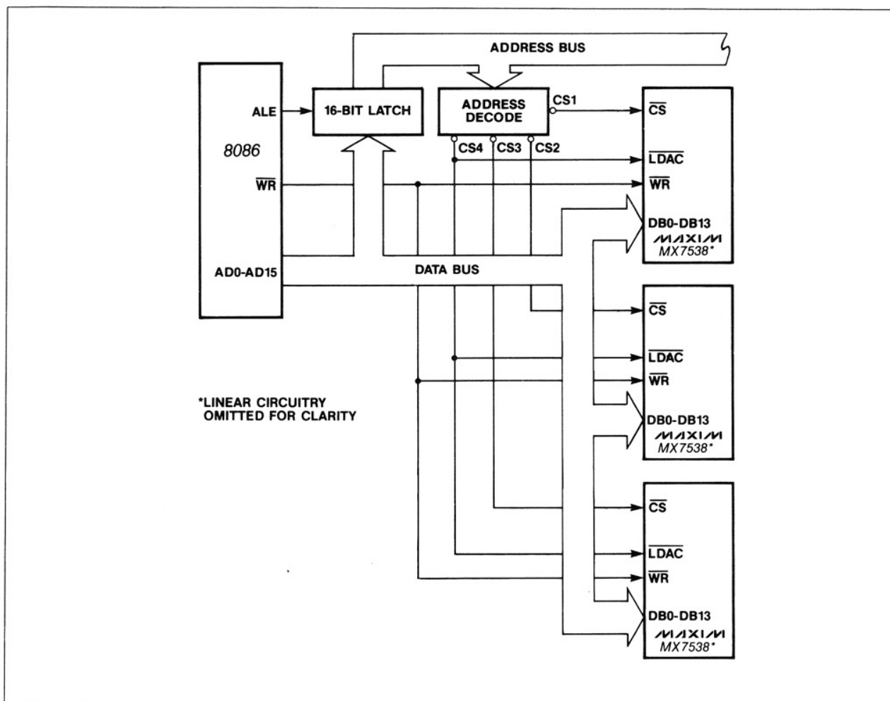
Figure 7. MX7538 - 8086 Interface: Multiple DAC System
