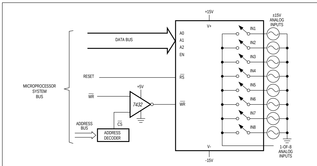
Figure 9. Bus Interface
