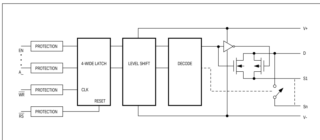
Figure 8. Simplified Internal Structure
