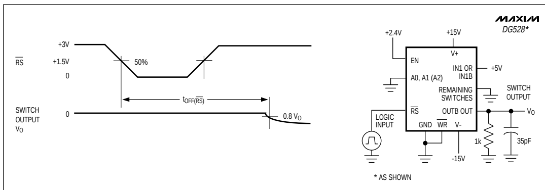
Figure 5. Reset Turn-Off Time t_{OFF(RS)} Test Circuit
