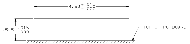
SUGGESTED PANEL CUTOUT NOT TO SCALE
