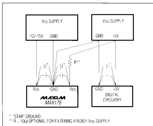
Figure 14. Power-Supply Grounding
