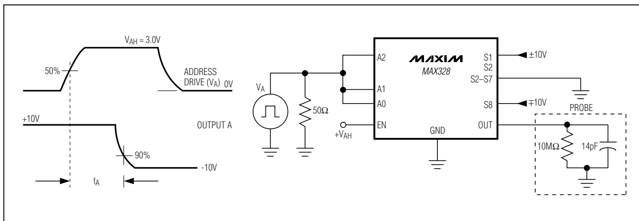
Figure 1. Access Time vs. Logic Level (High)
