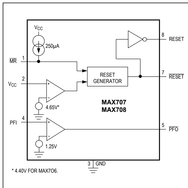
Figure 2. MAX707/MAX708 Block Diagram
