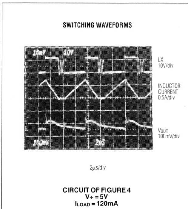
Figure 8. MAX734 Switching Waveforms
