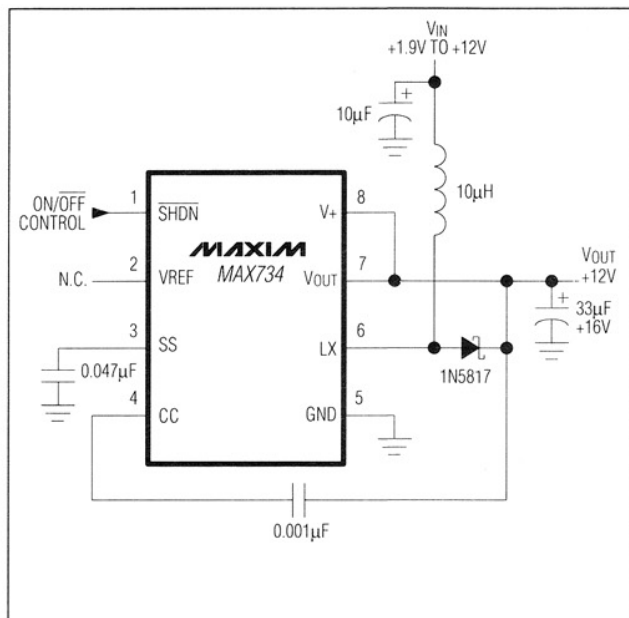
Figure 3. Bootstrap Operation
