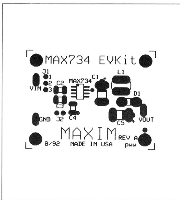
Figure 5. Component Placement Diagram (1x Scale)
