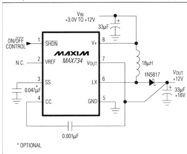
Figure 1. Standard Operating Circuit
