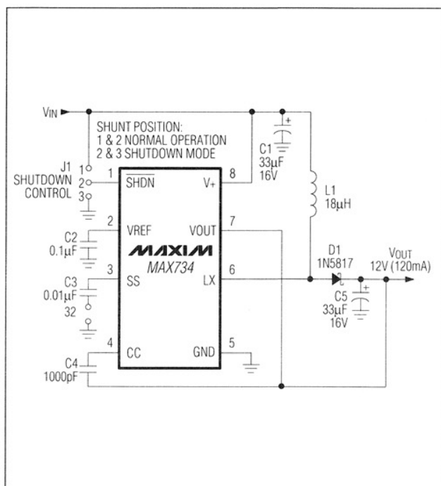
Figure 4. MAX734 EV Kit Schematic Diagram
