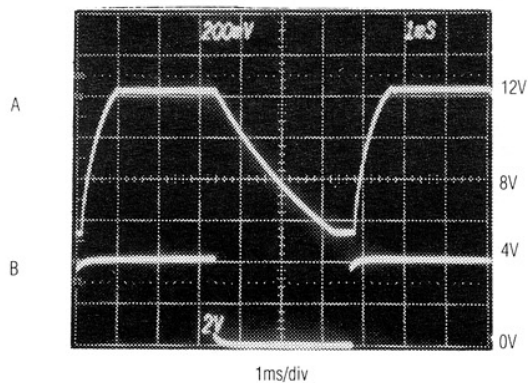
SHDN RESPONSE TIME
