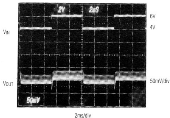
LINE-TRANSIENT RESPONSE
