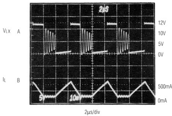
SWITCHING WAVEFORMS - DISCONTINUOUS CONDUCTION
