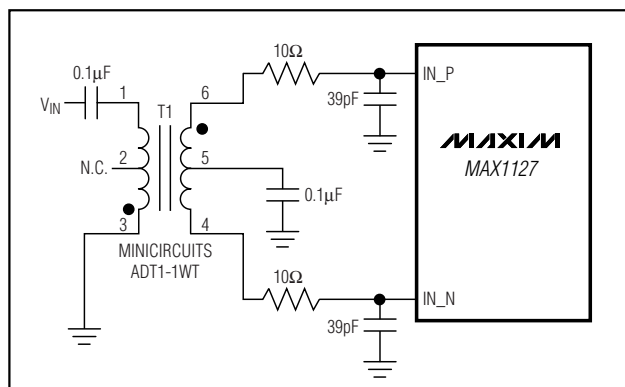
Figure 10. Transformer-Coupled Input Drive
