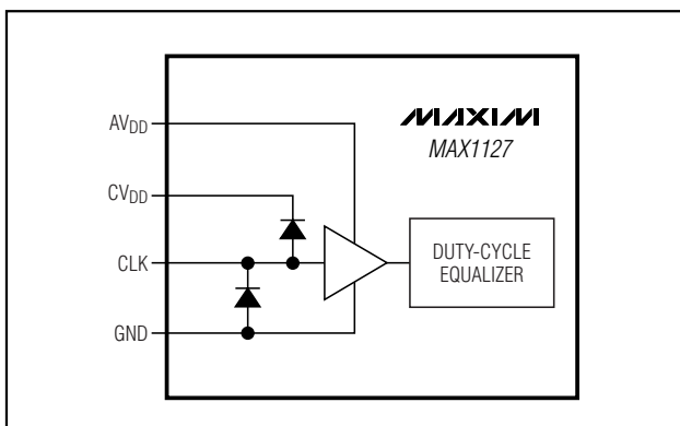
Figure 2. Clock Input Circuitry
