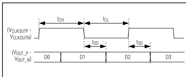
Figure 5. Serialized Output Detailed Timing Diagram
