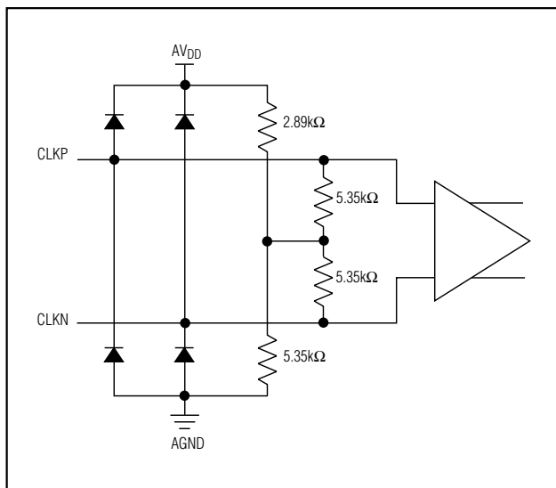
Figure 4. Simplified Clock Input Architecture
