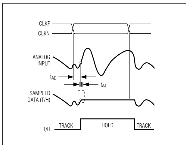
Figure 11. Aperture Jitter/Delay Specifications
