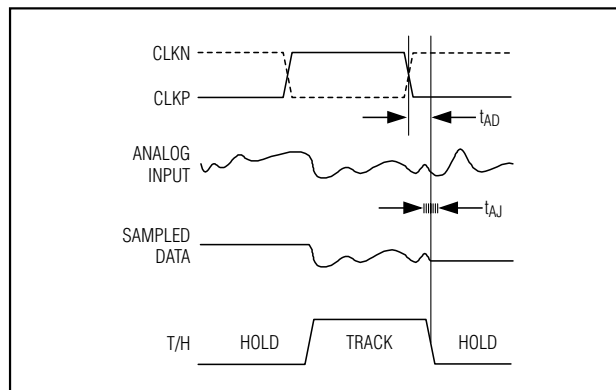
Figure 14. T/H Aperture Timing
