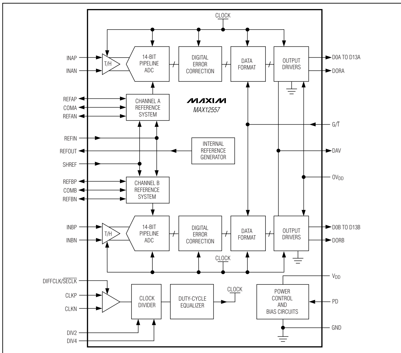
Figure 2. Functional Diagram
