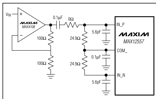
Figure 11. Single-Ended, AC-Coupled Input Drive
