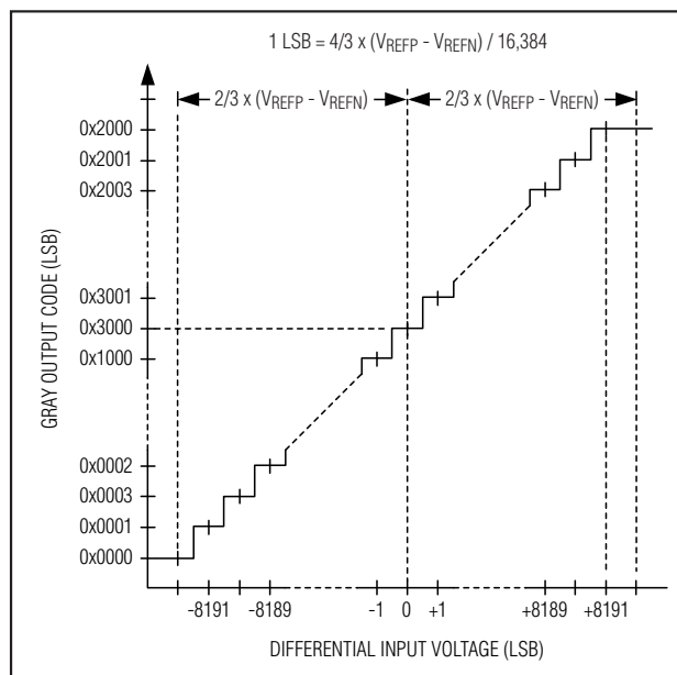
Figure 7. Gray-Code Transfer Function ( G/T = 1 )
