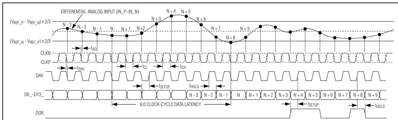
Figure 5. System Timing Diagram
