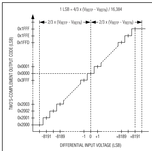
Figure 6. Two's-Complement Transfer Function ( G/T = 0 )
