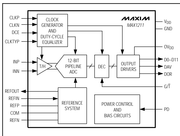
Figure 2. Functional Diagram
