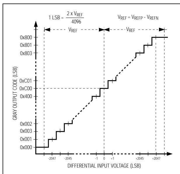
Figure 7. Gray Code Transfer Function ( G/\bar{T} = 1 )
