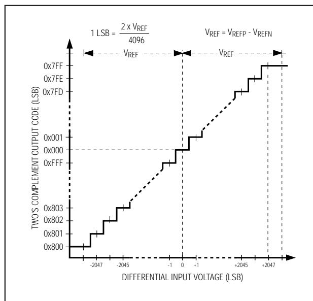
Figure 6. Two's Complement Transfer Function ( G/\bar{T} = 0 )
