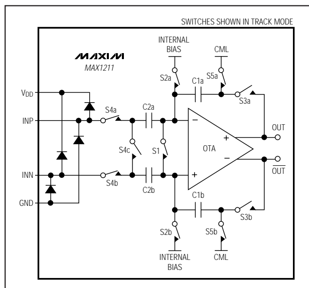
Figure 3. Internal T/H Circuit
