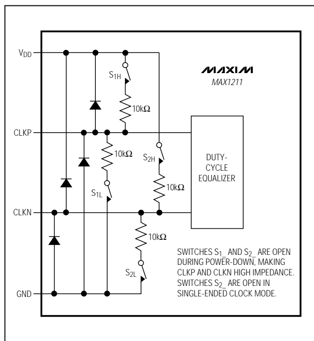
Figure 4. Simplified Clock Input Circuit
