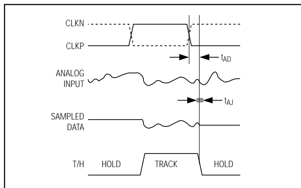
Figure 14. T/H Aperture Timing
