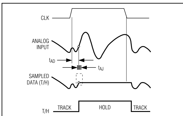
Figure 11. T/H Aperture Timing
