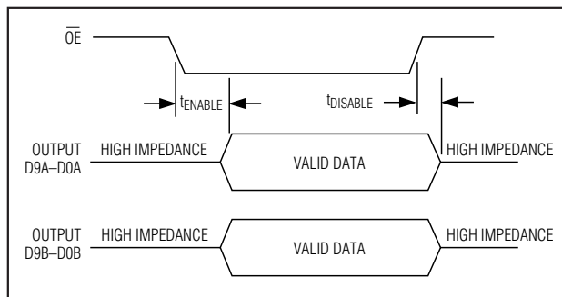
Figure 4. Output Timing Diagram
