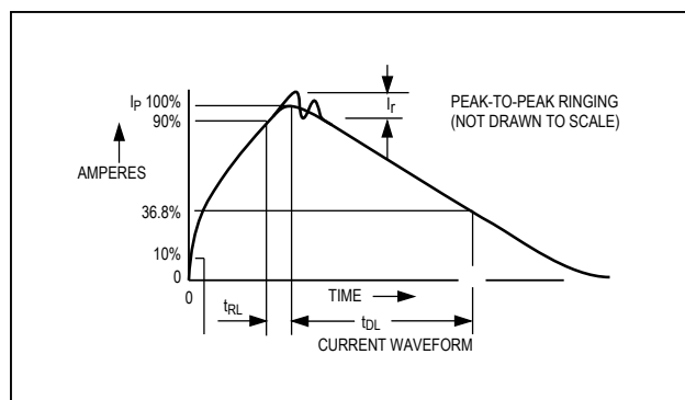
Figure 9b. Human Body Model Current Waveform
