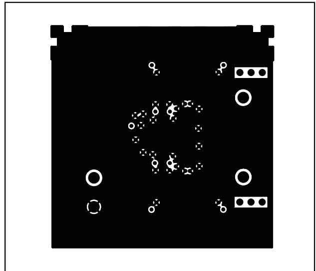
Figure 7. MAX2021 EV Kit PCB Layout—Inner Layer 2 (GND)
