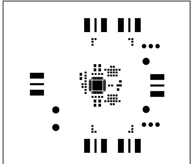
Figure 5. MAX2021 EV Kit PCB Layout—Top Soldermask
