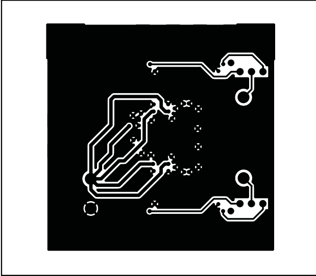
Figure 8. MAX2021 EV Kit PCB Layout—Inner Layer 3 (Routes)
