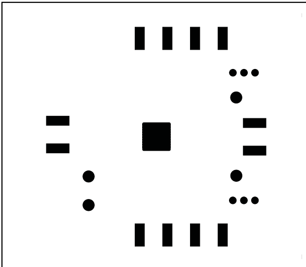
Figure 10. MAX2021 EV Kit PCB Layout—Bottom Soldermask
