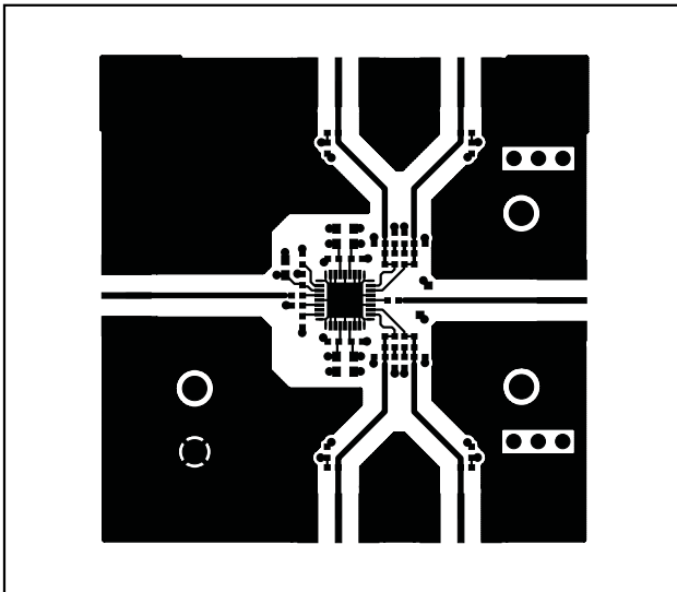
Figure 6. MAX2021 EV Kit PCB Layout—Top Layer Metal
