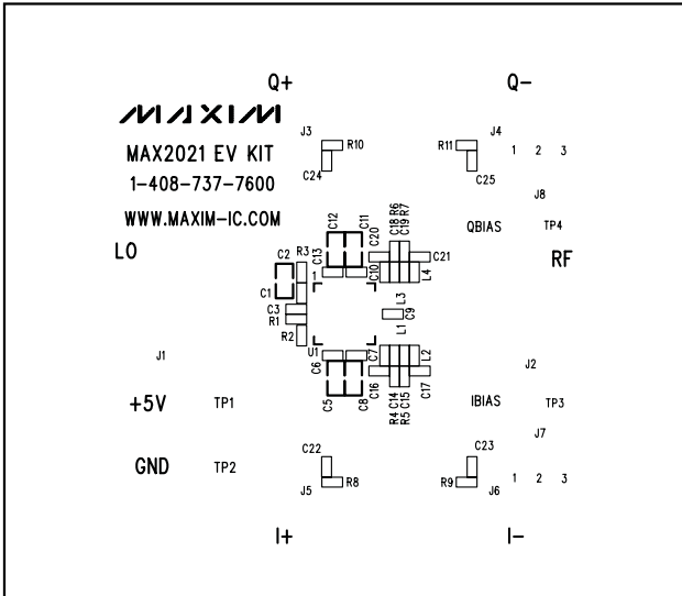
Figure 4. MAX2021 EV Kit PCB Layout—Top Silkscreen
