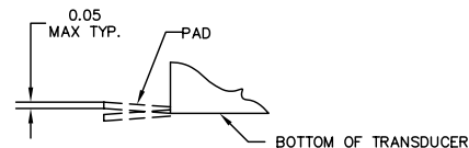
DETAIL - "A"
