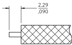
RG402 CABLE STRIP
