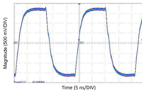
Figure 21. DS90UR124 PCLK Output at 43 MHz
