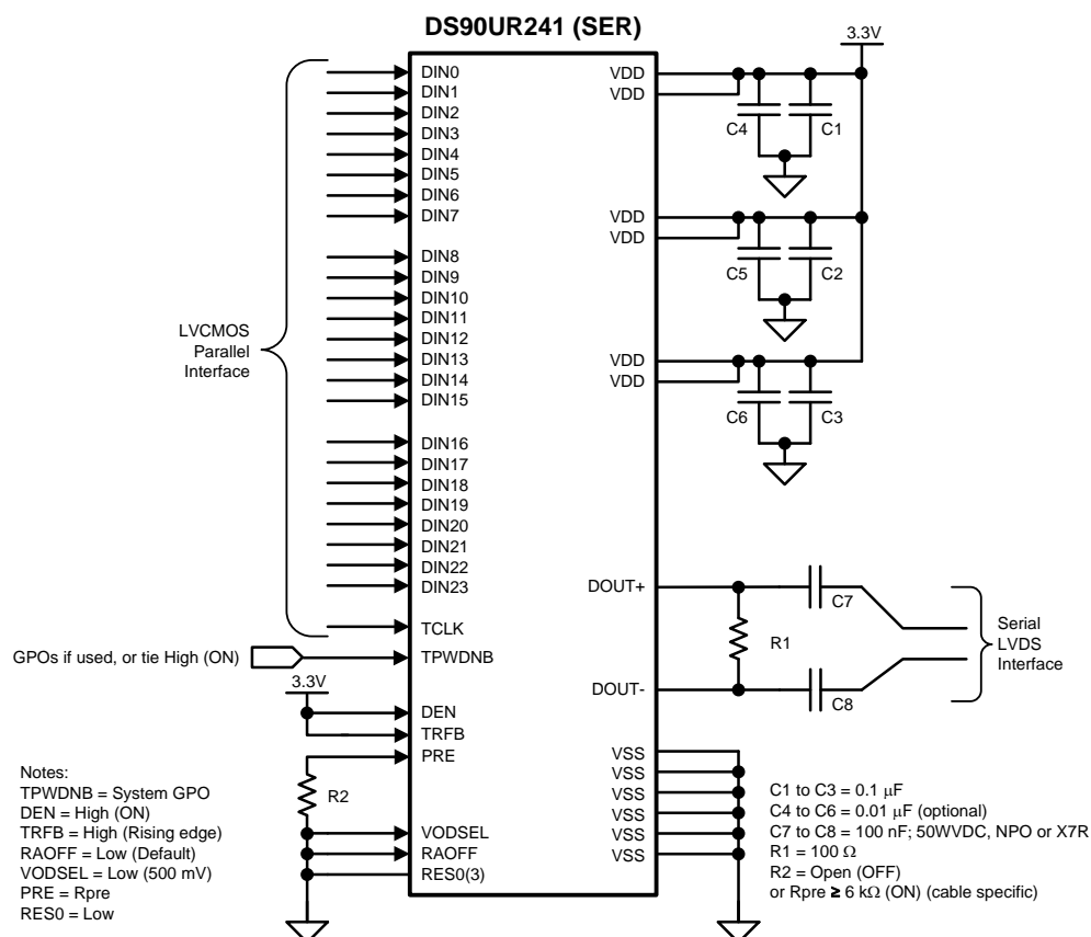
Figure 22. DS90UR241 Connection Diagram
