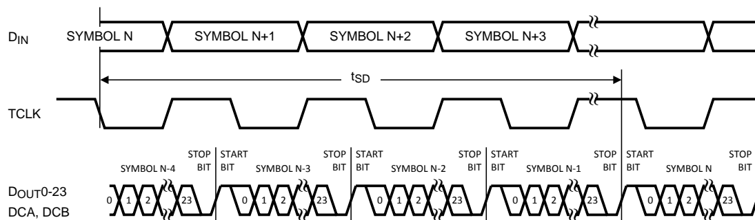
Figure 10. Serializer Delay
