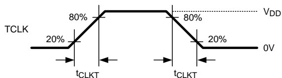
Figure 6. Serializer Input Clock Transition Times
