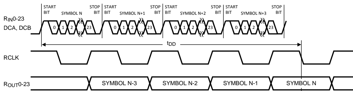
Figure 14. Deserializer Delay
