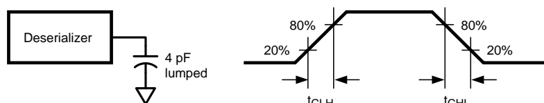
Figure 13. Deserializer LVCMOS Output Load and Transition Times
