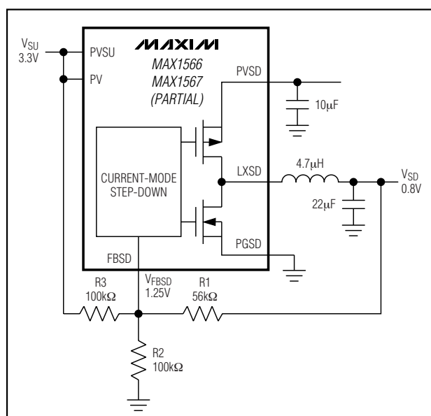
Figure 18. Setting PVSD for Outputs Below 1.25V
