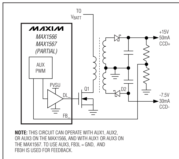
Figure 9. +15V and -7.5V CCD Bias with Transformer
