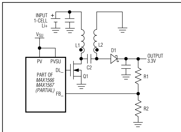
Figure 13. SEPIC Converter Additional Boost-Buck Channel
