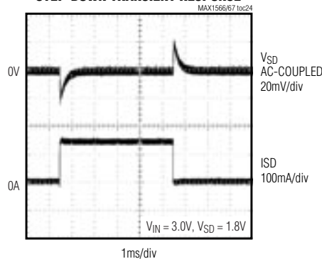
STEP-DOWN TRANSIENT RESPONSE
