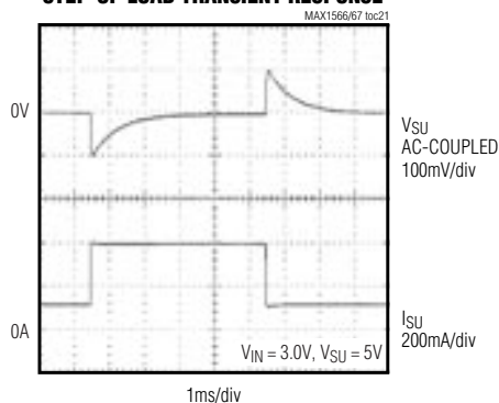
STEP-UP LOAD TRANSIENT RESPONSE
