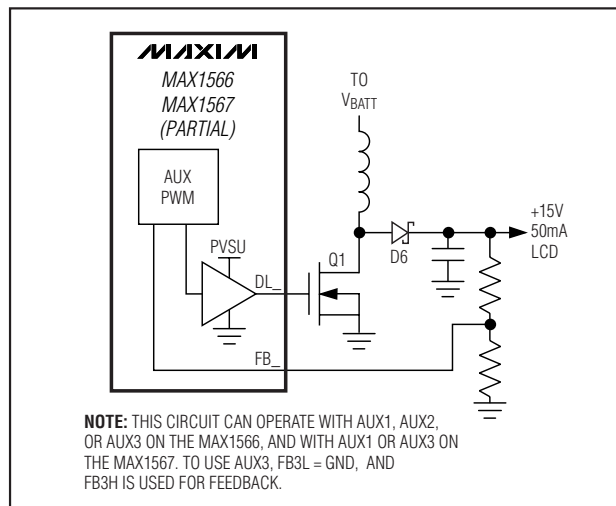
Figure 8. +15V LCD Bias with Basic Boost Topology
