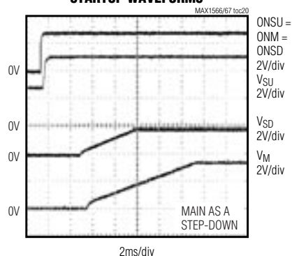
MAIN (STEP-DOWN MODE) AND STEP-DOWN STARTUP WAVEFORMS
