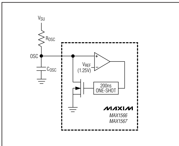
Figure 6. Oscillator Functional Diagram
