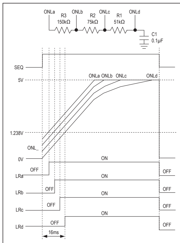
Figure 6. Single-Capacitor Sequence Configuration
