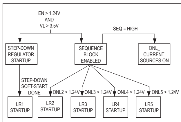
Figure 5. Startup Conditions
