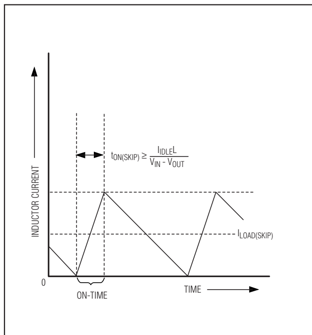
Figure 4. Pulse-Skipping/Discontinuous Crossover Point
