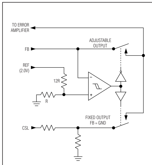
Figure 5. Dual-Mode Feedback Decoder
