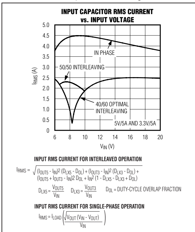
Figure 10. Input RMS Current
