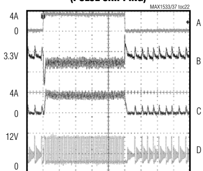
3.3V OUTPUT LOAD TRANSIENT (PULSE SKIPPING)
