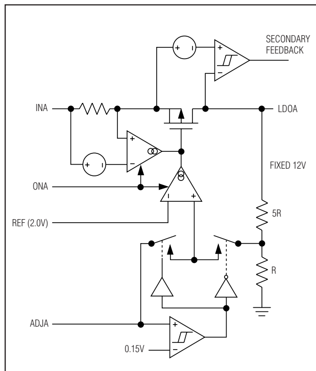
Figure 8. Linear-Regulator Functional Diagram
