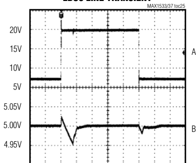
LDO5 LINE TRANSIENT
