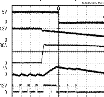
OUTPUT OVERLOAD (UVP ENABLED)
