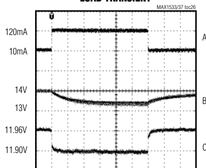
AUXILIARY LINEAR-REGULATOR LOAD TRANSIENT
