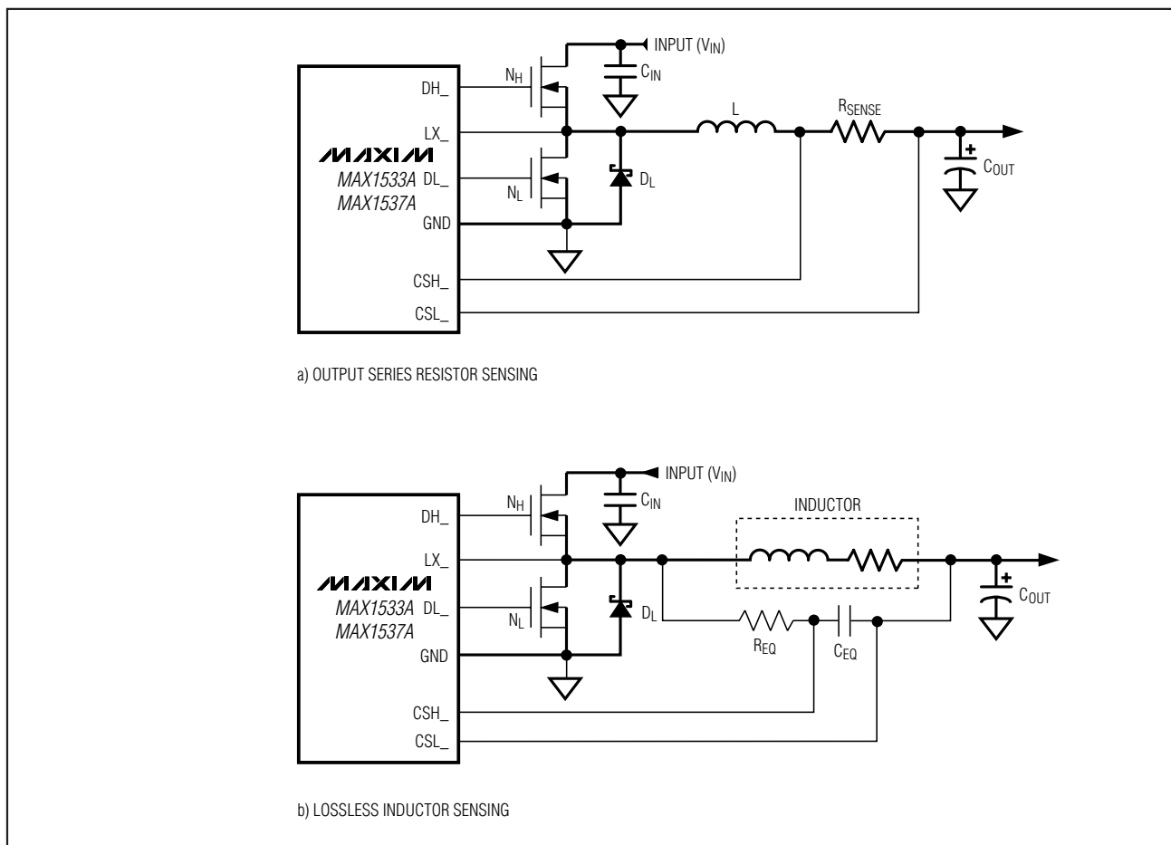
Figure 9. Current-Sense Configurations
