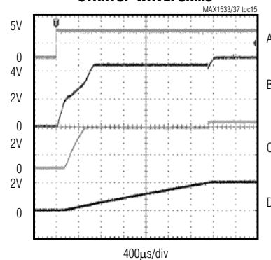
LINEAR-REGULATOR STARTUP WAVEFORMS
