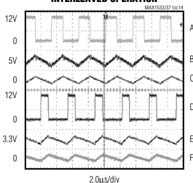
INTERLEAVED OPERATION
