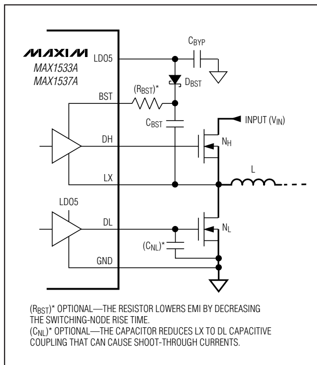
Figure 6. Optional Gate-Driver Circuitry
