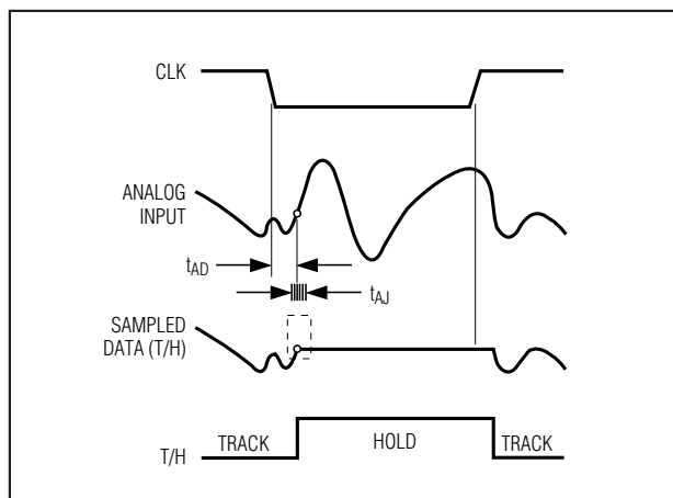
Figure 12. T/H Aperture Timing
