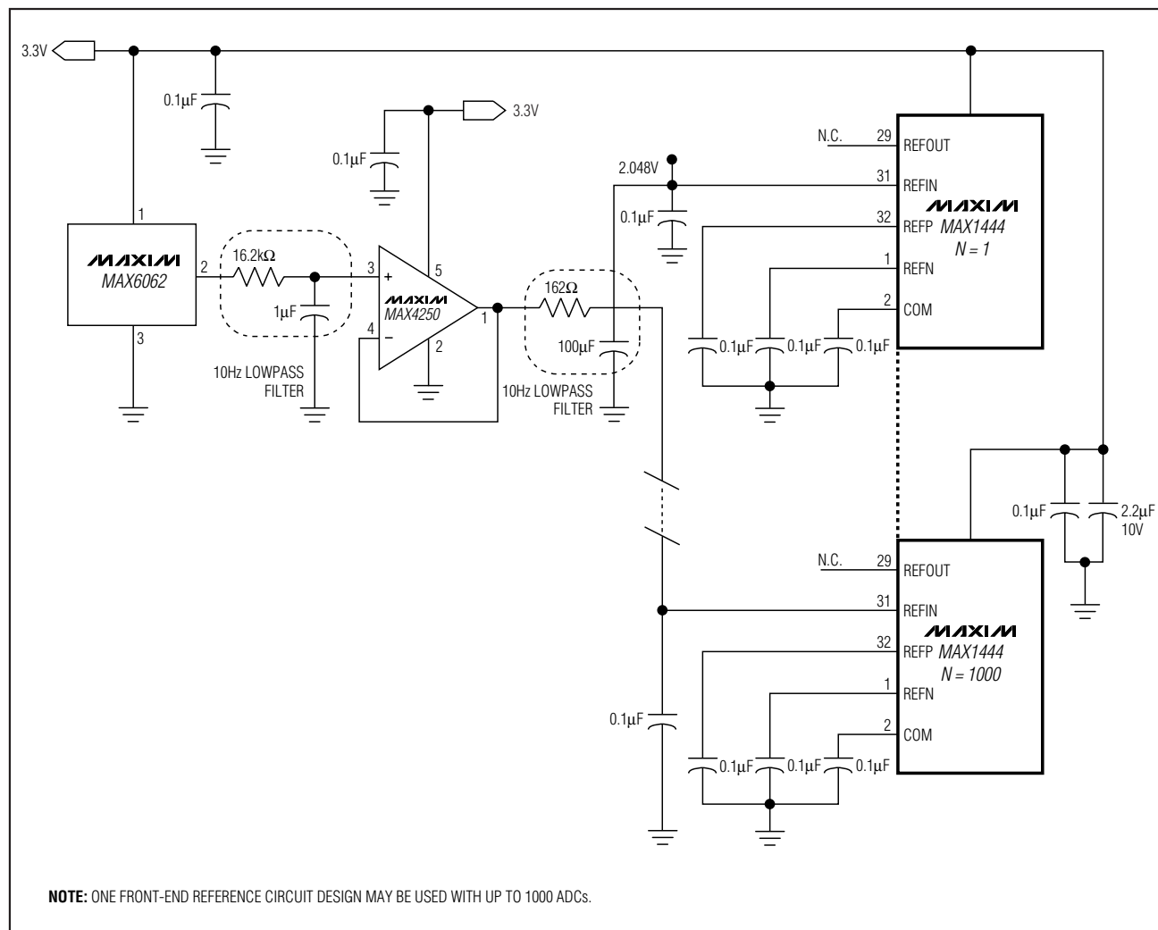
Figure 10. Buffered External Reference Drives Up to 1000 ADCs
