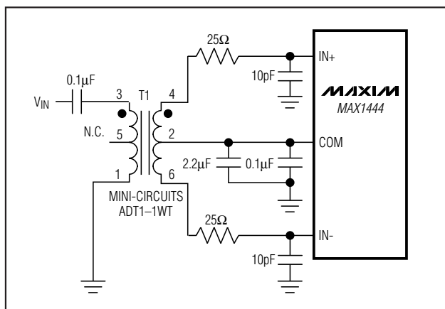
Figure 8. Using a Transformer for AC Coupling
