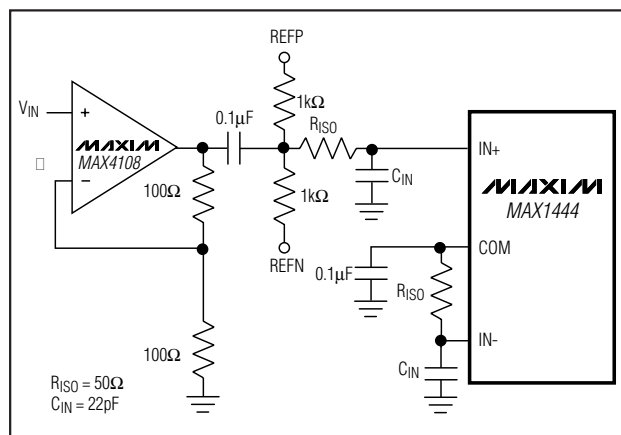
Figure 9. Single-Ended AC-Coupled Input
