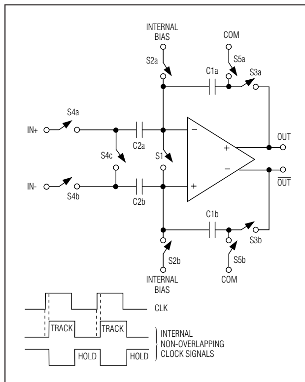
Figure 2. Internal T/H Circuit
