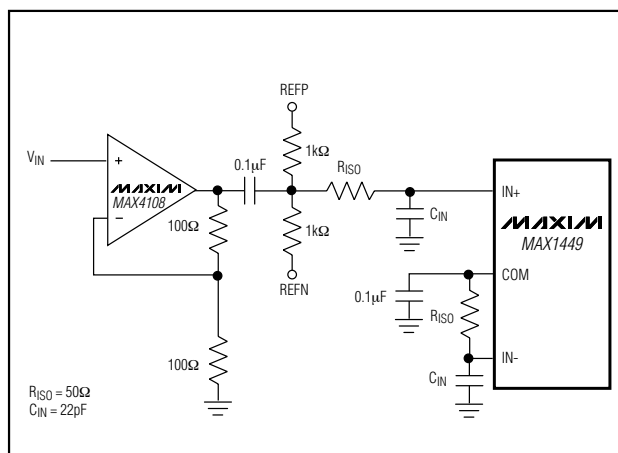
Figure 9. Single-Ended AC-Coupled Input
