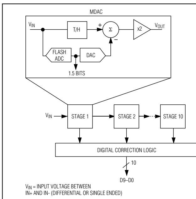
Figure 1. Pipelined Architecture—Stage Blocks
