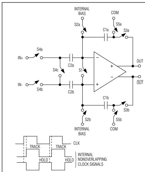
Figure 2. Internal T/H Circuit
