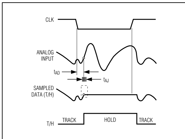
Figure 12. T/H Aperture Timing
