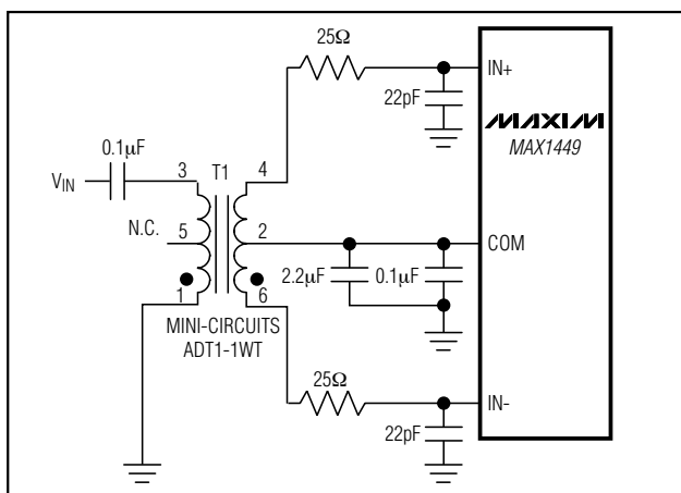
Figure 8. Using a Transformer for AC-Coupling
