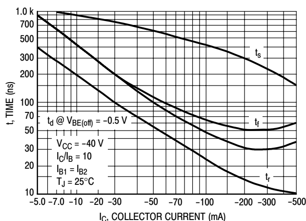
Figure 4. Switching Time
