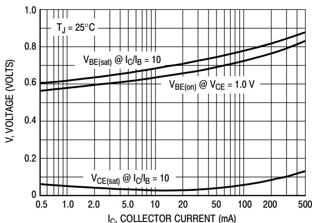
Figure 7. "On" Voltages
