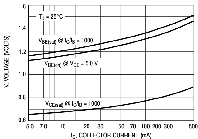
Figure 10. "On" Voltages
