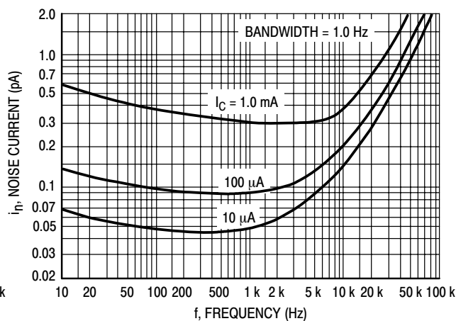
Figure 3. Noise Current
