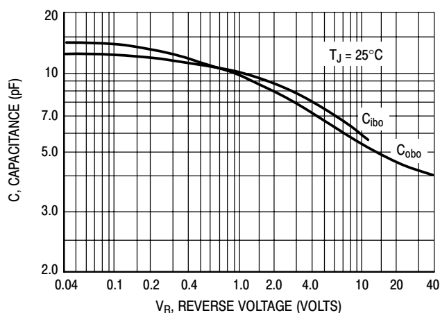
Figure 6. Capacitance
