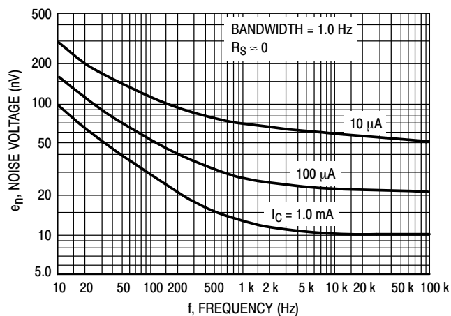
Figure 2. Noise Voltage
