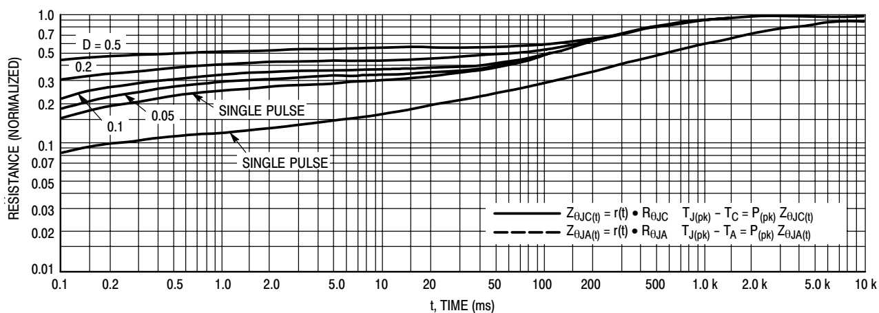
Figure 12. Thermal Response
