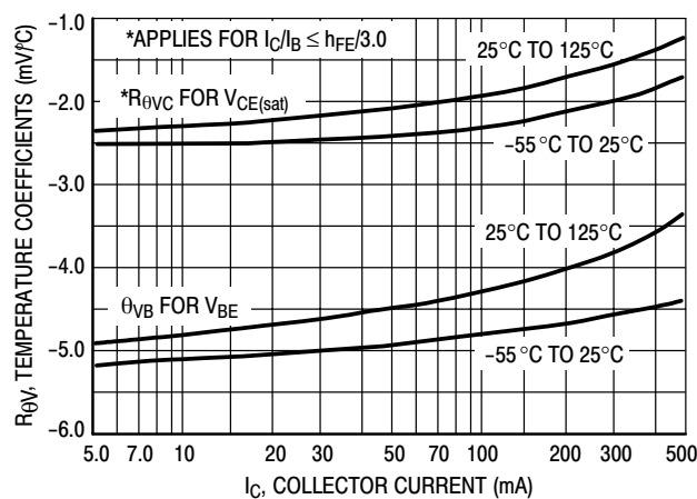
Figure 11. Temperature Coefficients
